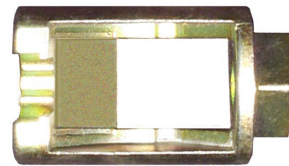
1/2" NPT RECESSED/CONCEALED WRENCH P/N 325391
